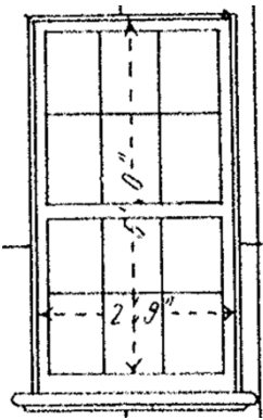
Window VR Goods Shed 5' 0" x 2' 9" Measurements inside of frame
