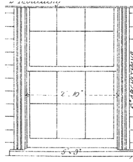
Window Gatekeepers Cottage 4' 7 1/2" x 2' 10" Measurements inside of frame Glass 12"x10"
