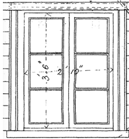
Window Gatekeepers Cottage 3' 6" x 2' 10"
