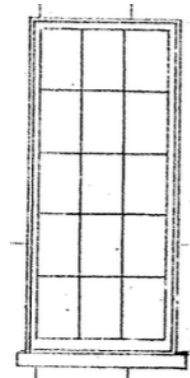
Window VR Engine Shed Benalla 6' 9" x 3' 1" Measurements inside of frame
