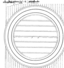
Louver Ventilator VR Engine Shed Benalla 3' 0'
