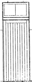
Door VR Goods Shed 7' 0' x 2' 8" x 1 1/2"
