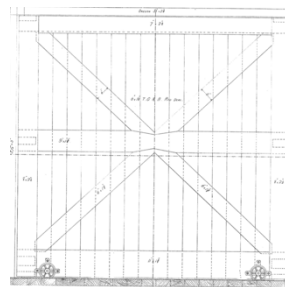
Door VR Goods Shed 7' 0' x 2' 8" x 1 1/2"
