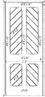
Door VR Engine Shed Dimboola 6' 9 1/2" x 2' 9"
