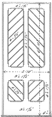
Door VR Engine Shed Dimboola 6' 10" x 2' 10"
